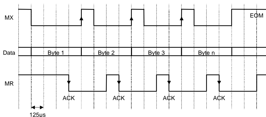
Figure 5 Monitor Handshake Timing (general case)
