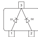
BAT64-05 BAT64-05W
