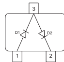
BAT64-04 BAT64-04W
