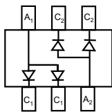
BAT54ADW* Marking: KL6
