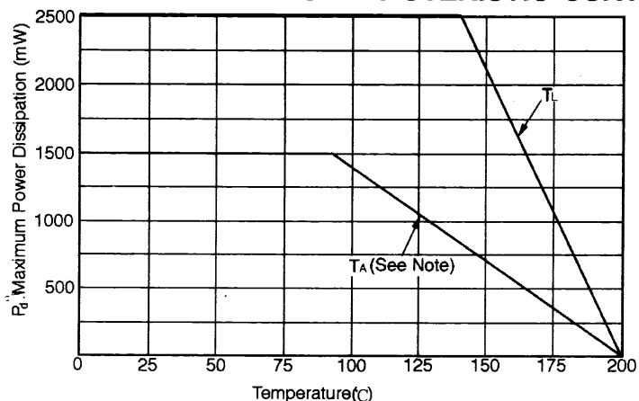
FIGURE 1 – Power Derating Curve
