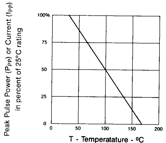
FIGURE 3 DERATING CURVE
