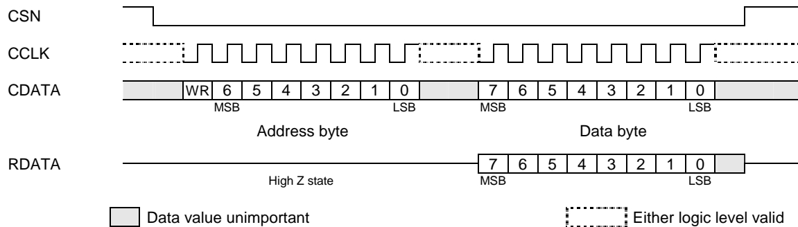
Figure 6 C-BUS Operation
