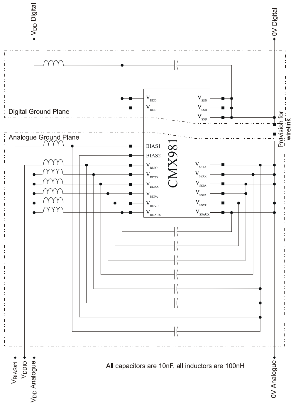
Figure 2 Recommended External Components
