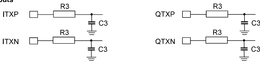
Figure 2b Recommended External Components - Tx Outputs
