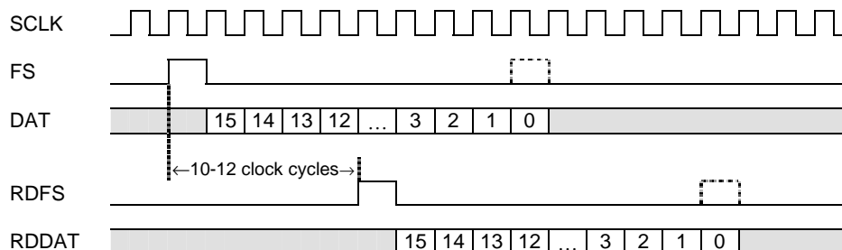
Figure 5 FSB Operation
