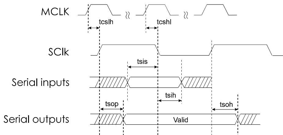
Figure 7 Serial Port Interfaces - Timing Parameters
