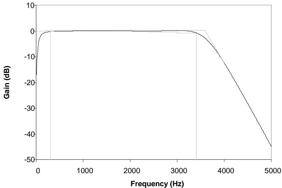
Figure 4 Voice Codec Filter Response
