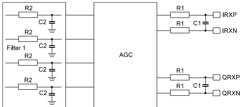
Figure 2a Recommended External Components - Rx Inputs
