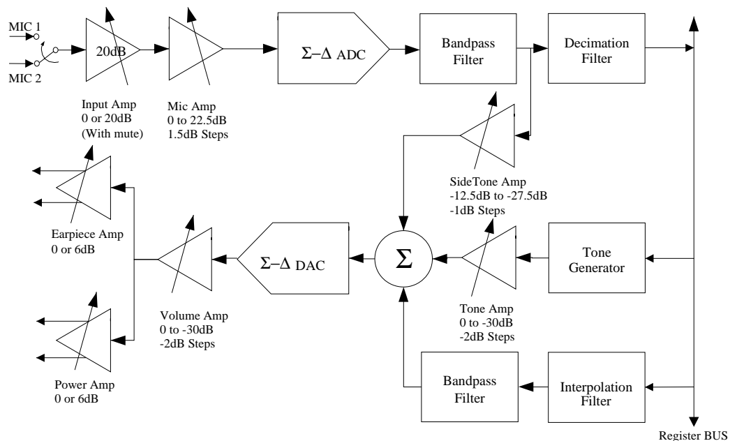
Figure 3 Voice Codec Block Diagram
