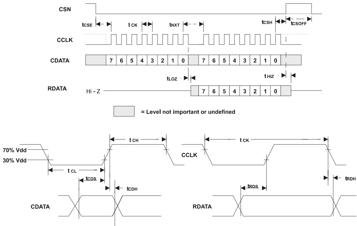
Figure 7f C-BUS Interface - Timing Parameters
