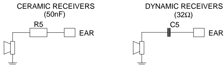
Figure 2e Recommended External Components - Codec Earpiece Output
