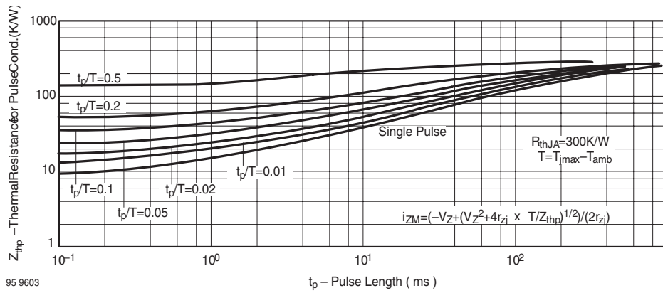
Figure 11. Thermal Response
