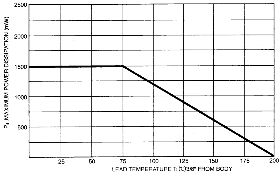
FIGURE 1 POWER DERATING CURVE
