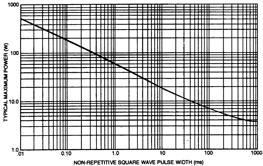
FIGURE 2 TRANSIENT SURGE CAPABILITY
