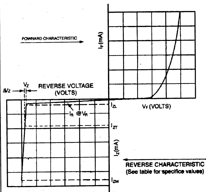
FIGURE 2 - ZENER DIODE CHARACTERISTICS AND SYMBOL IDENTIFICATION
