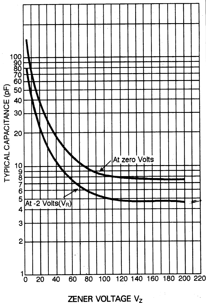
FIGURE 3 - CAPACITANCE VS. V_z CURVE
