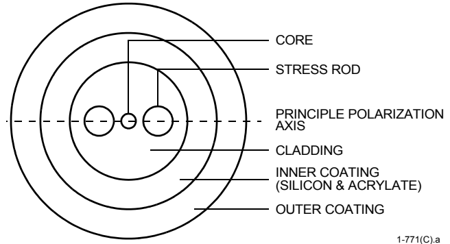
Figure 1. Polarization-Maintaining Fiber
