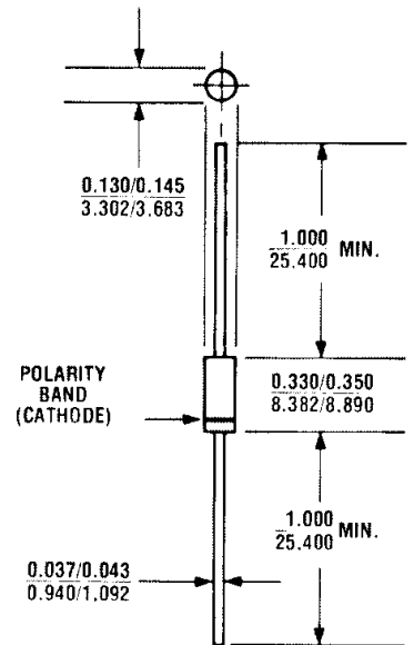
FIGURE 1 All dimensions in INCH m.m.
