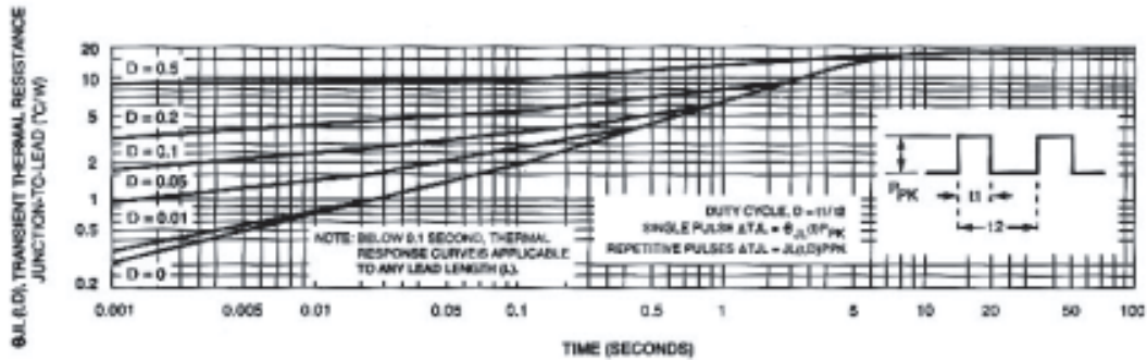
Figure 3. Typical Thermal Response
