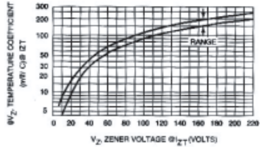
Figure 2. Temperature Coefficient-Range for Units 6 to 220 Volts
