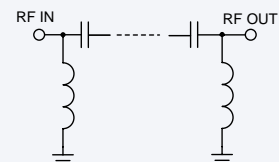
schematic B
