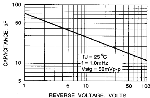
FIG. 5 - TYPICAL JUNCTION CHARACTERISTICS
