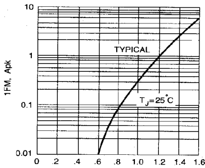
Fig. 3 - FORWARD CHARACTERISTICS
