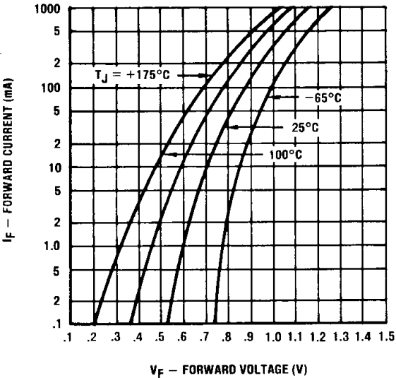
FIGURE 2 FORWARD VOLTAGE vs. FORWARD CURRENT
