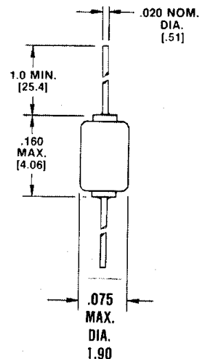
FIGURE 1B PACKAGE D0-35
