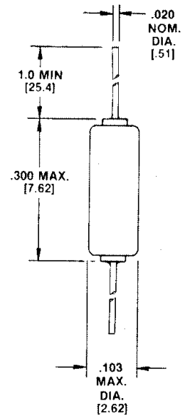
FIGURE 1A PACKAGE D07
