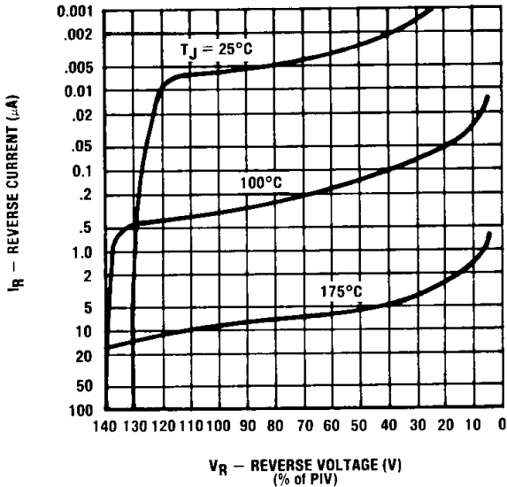
FIGURE 3 REVERSE VOLTAGE vs. REVERSE CURRENT
