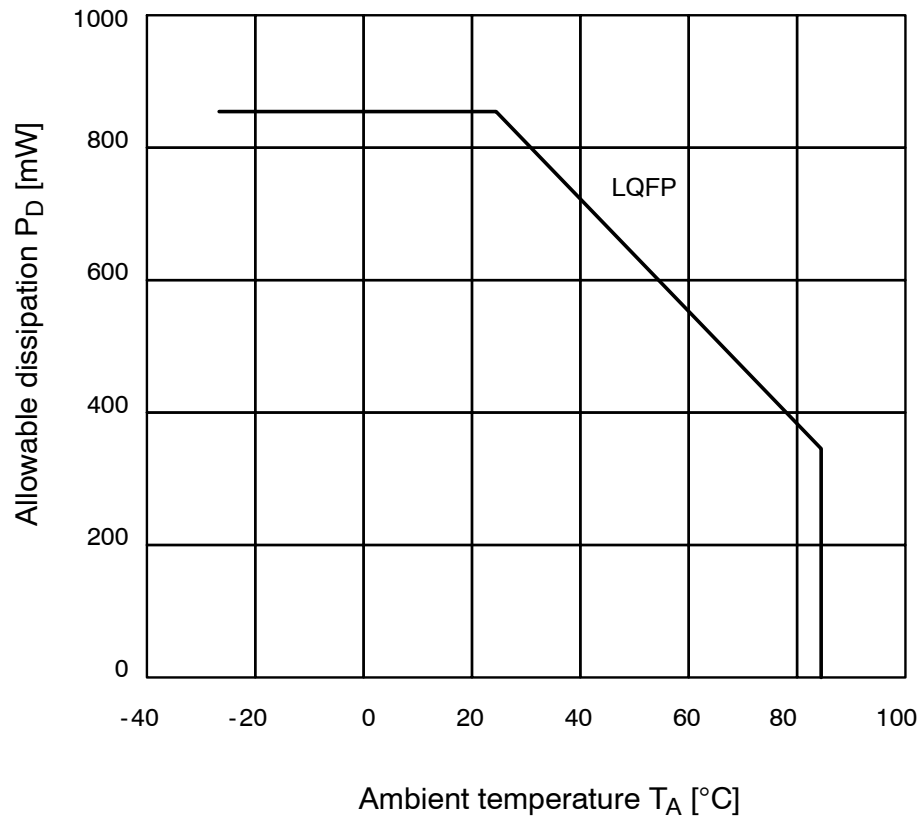
Allowable dissipation vs. ambient temperature curve
