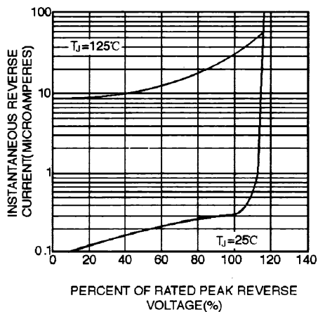
FIG. 4 - TYPICAL REVERSE CHARACTERISTICS PER ELEMENT
