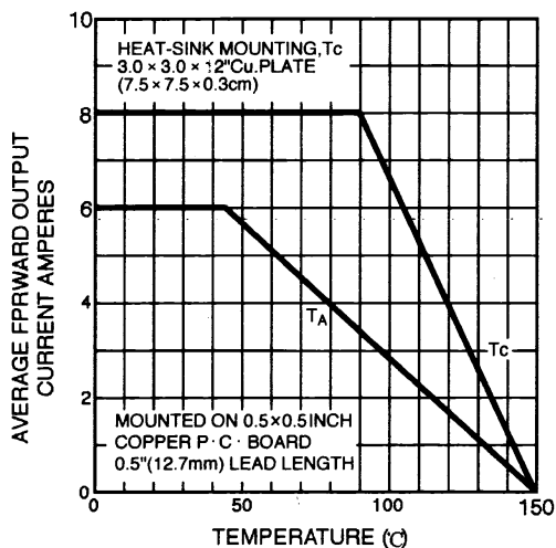
FIG. 2 - TYPICAL FORWARD OUTPUT CURRENT DERATING CURVE
