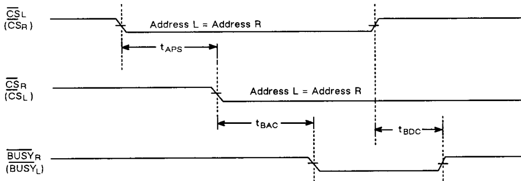
Data Contention Cycle No. 2 ( \overline{CS} Controlled) 1, 3 :
