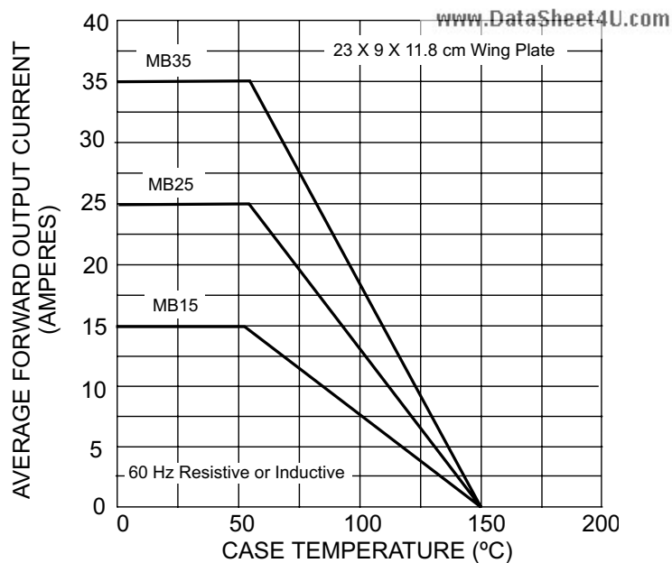
Fig. 2 Maximum Output Rectified Current
