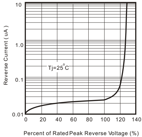
Fig. 1 - Reverse Characteristics
