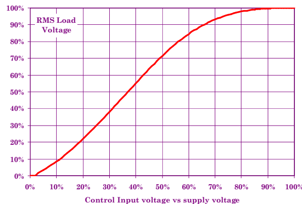
RMS Load Voltage Ratio vs. Input
