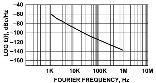
Figure 6. VTO-9068 Normalized Phase Noise @ 1360 MHz S.S.B. Power Spectral Density.
