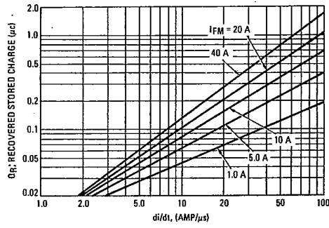
FIGURE 13 - T J = 75°C
