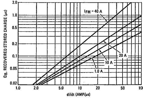
FIGURE 15 - T J = 150°C
