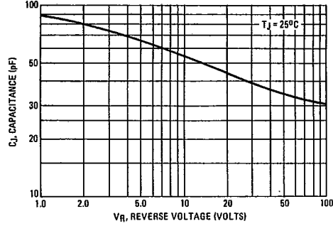
FIGURE 11 - JUNCTION CAPACITANCE
