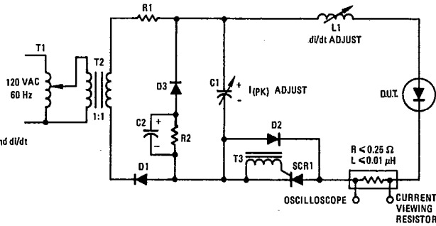
FIGURE 16 — JEDEC REVERSE RECOVERY CIRCUIT
