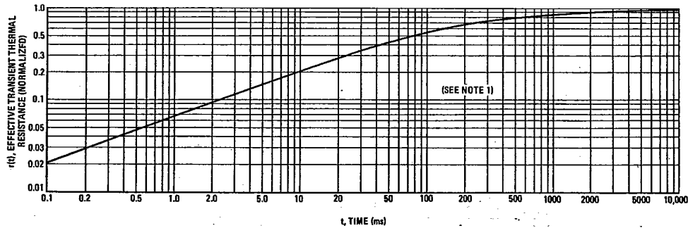
FIGURE 3 - THERMAL RESPONSE
