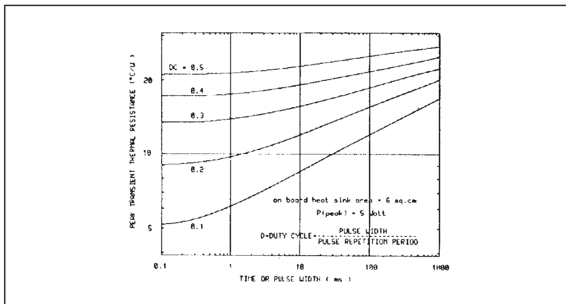
Figure 36: Peaktransient Rth pulse width and Duty Cycle.
