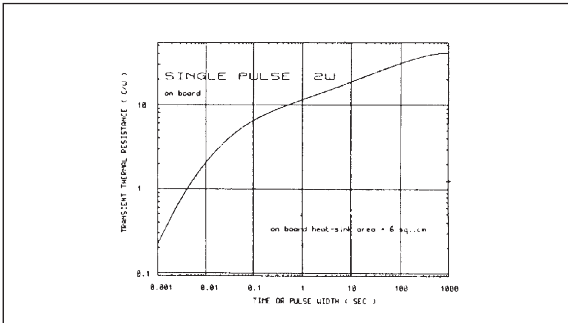
Figure 35: Transient thermal resistance for single pulses
