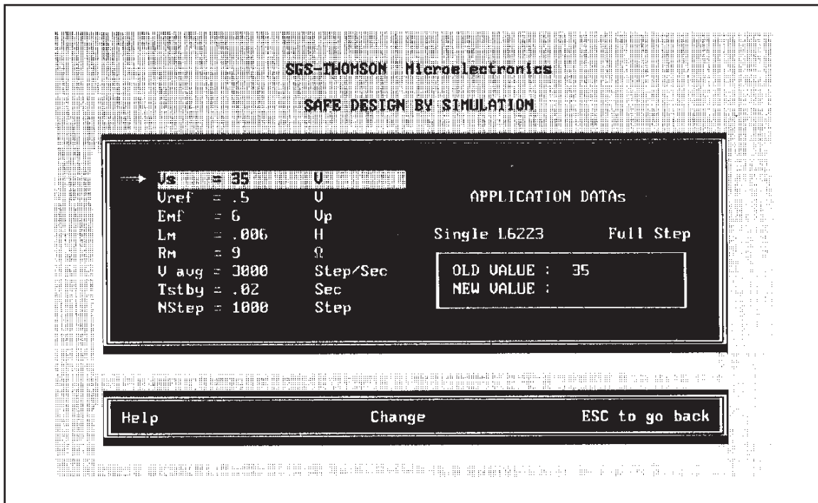
Figure 29a: Single L6223 high speed, Application Data.
