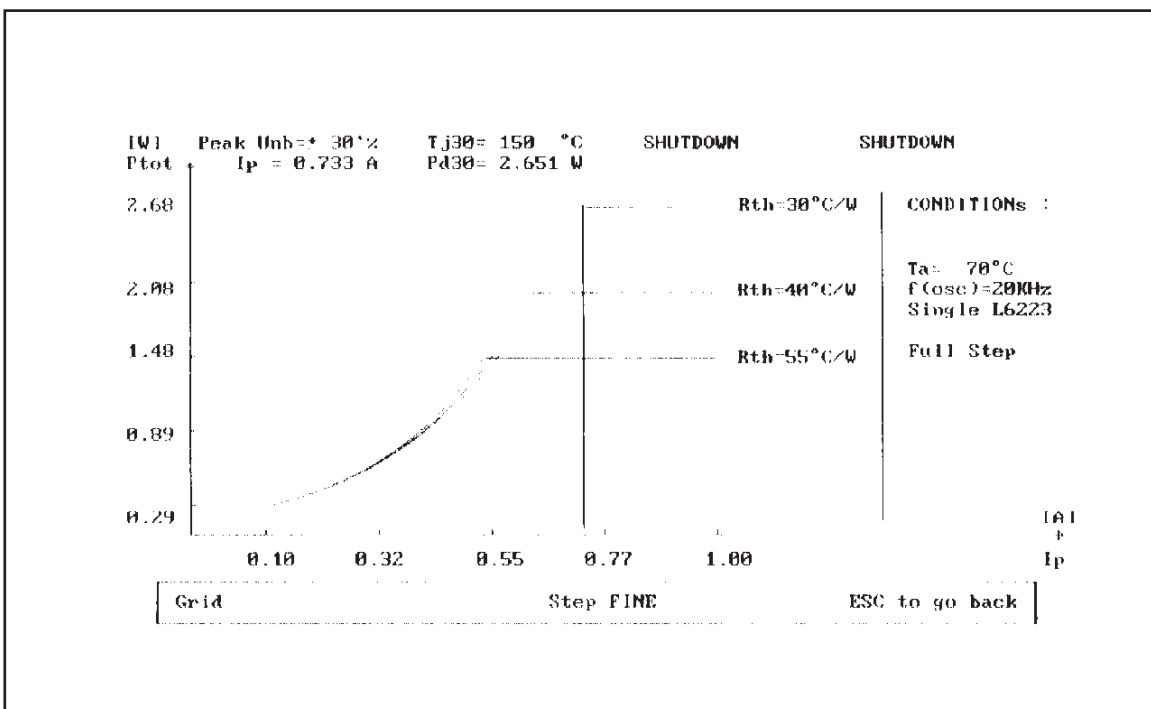
Figure 29b: Total Power Dissipation.
