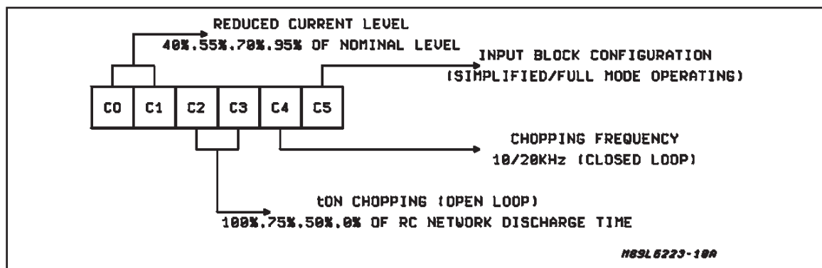
Figure 7: Internal Six-Bit Shift Register Bit Functions
