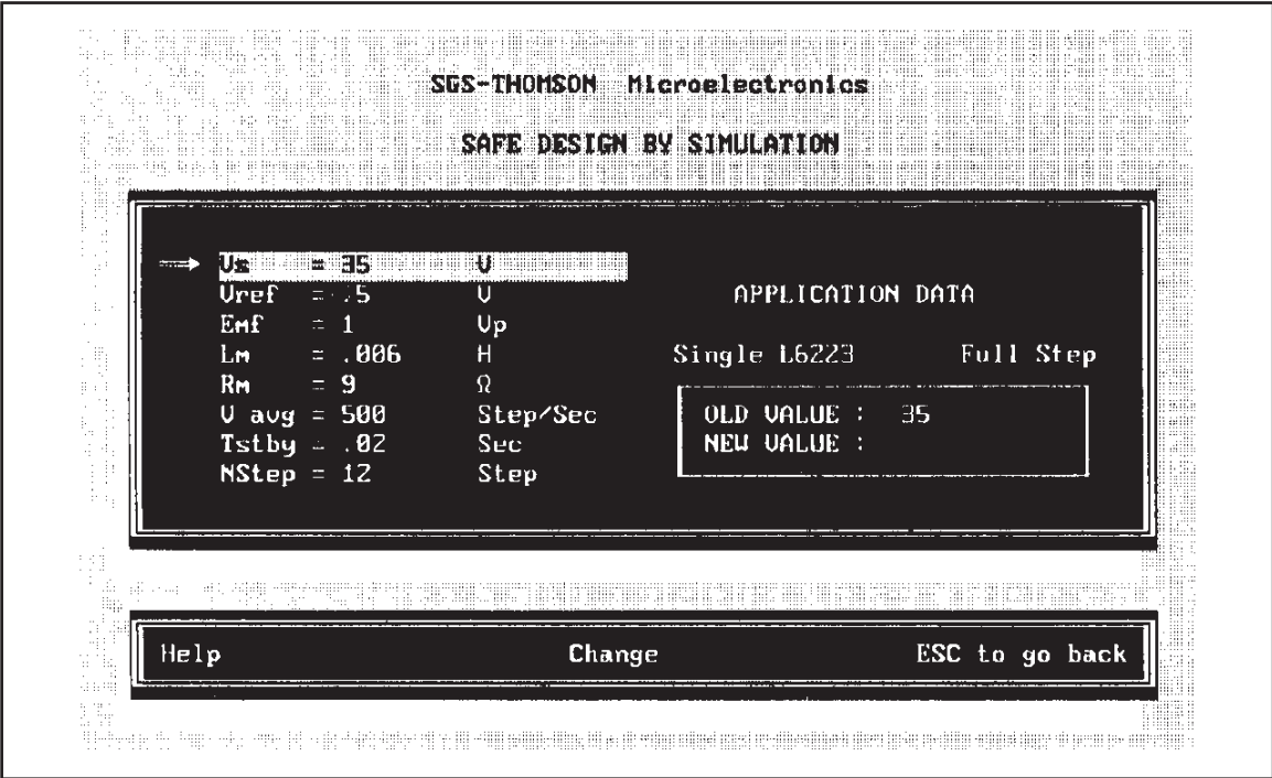
Figure 28a: Single L6223 slow speed, Application Data.
