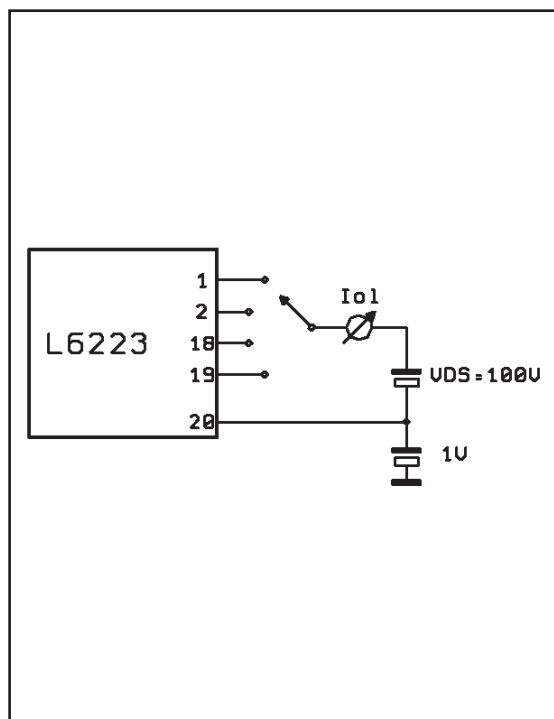
Figure 1: Output leakage I OL Test Circuit
