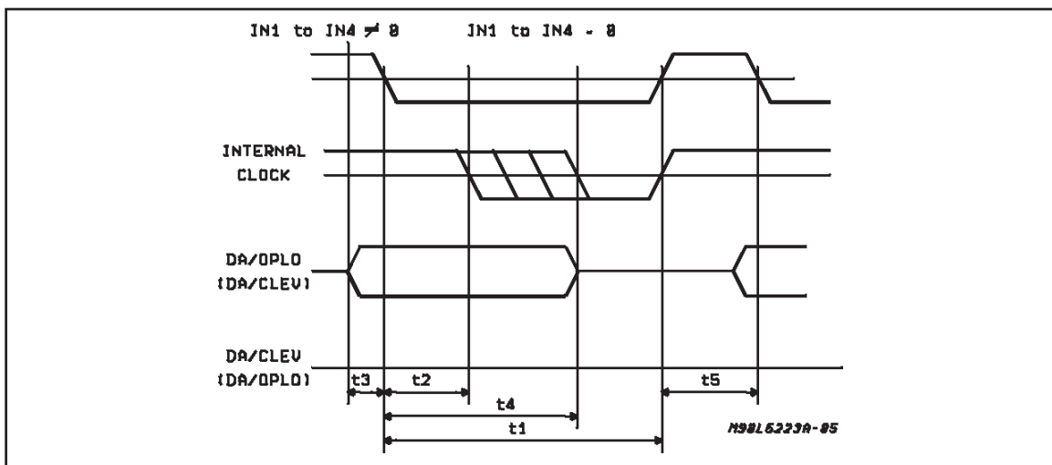
Figure 6: Programming Timing Diagram (see Block Diagram)
