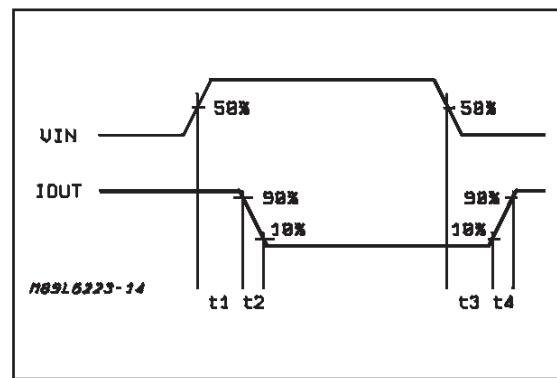
Figure 5: Output Sink Current Delay vs Input Control
