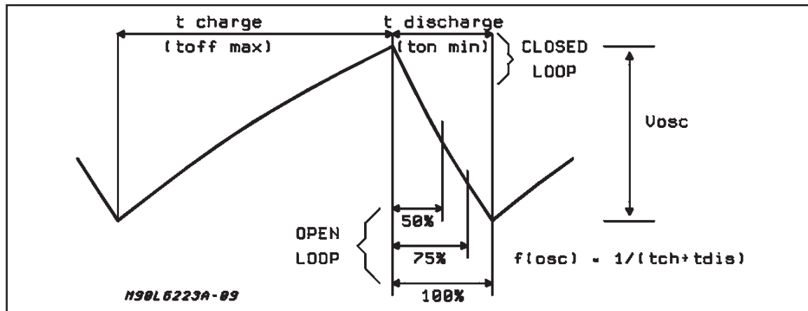
Figure 20: Oscillator waveform and timing.
