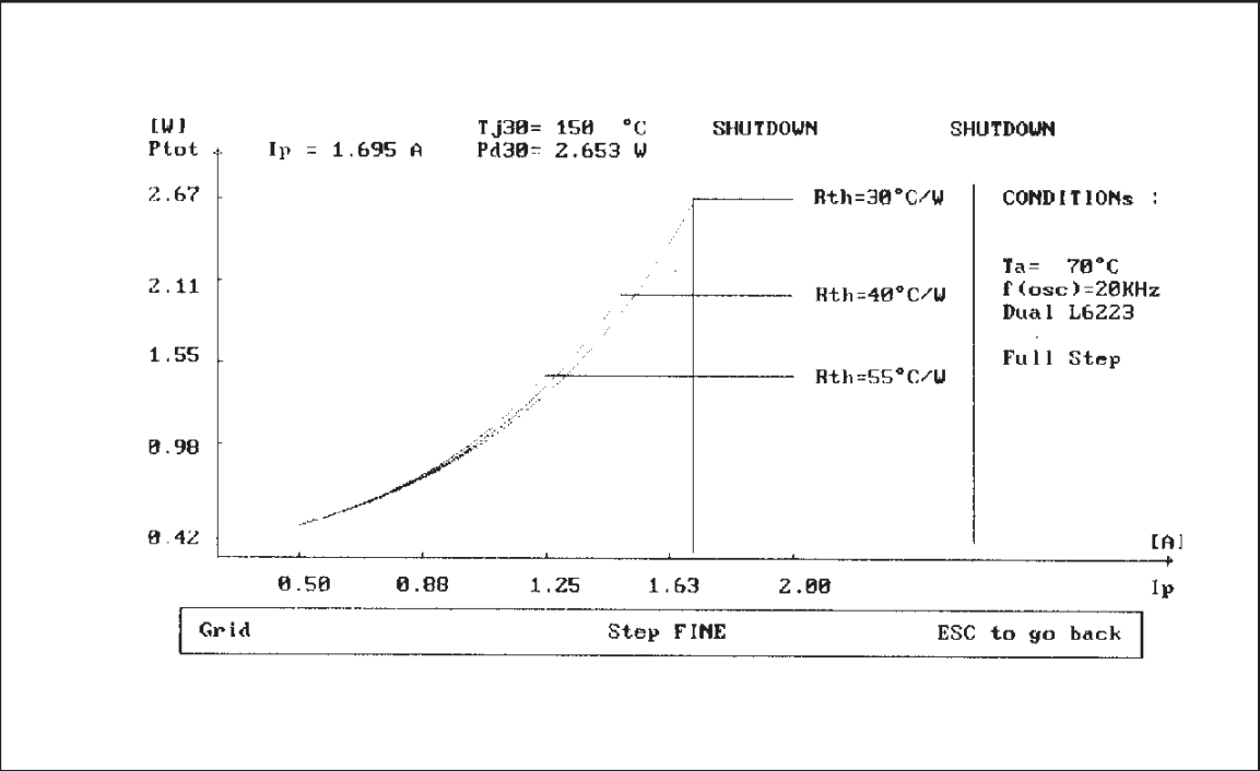
Figure 30b: Total Power Dissipation.
