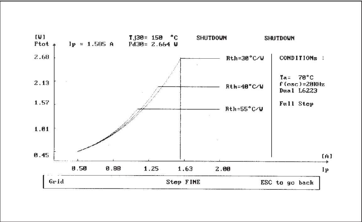
Figure 31b: Total Power Dissipation.
