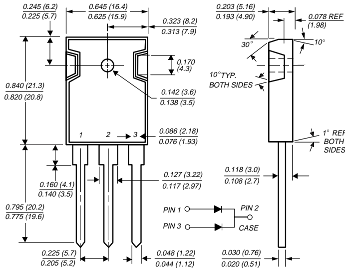
TO-247AD (TO-3P)
