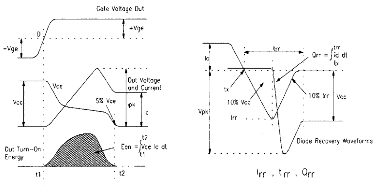
Fig. 18 - Test Waveforms for Circuit of Fig. 16, Defining E_{ON} , E_{REC} , t_{D(ON)} , t_r , I_{RR} , I_{RR} , Q_{RR}
