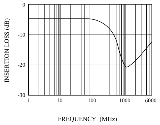
Fig. 2 S_{21} - F
