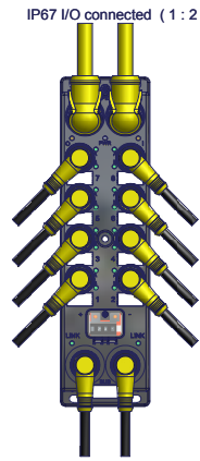
IP67 I/O connected (1:2) Window open (105°)
