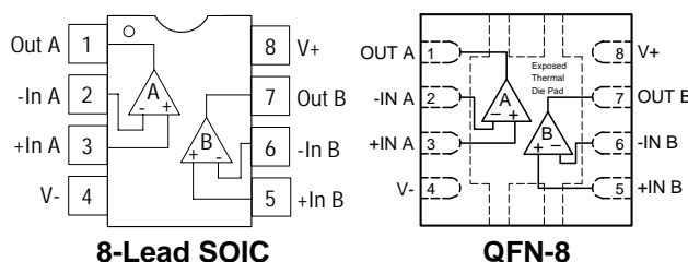
CS3004 (Top View)
