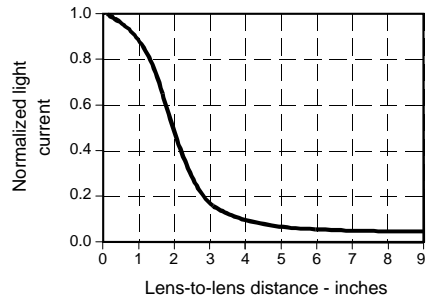
Fig. 7 Coupling Characteristics SE5450 with SD5443
