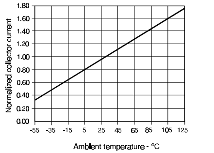
Fig. 8 Collector Current vs Ambient Temperature
