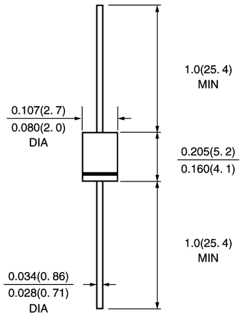
DO-41\DO-204AL
