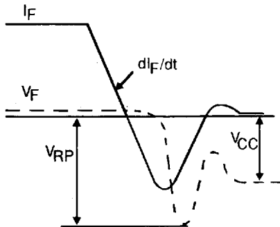
Figure 12 : Turn-off switching characteristics (with series inductance). www.DataSheet4U.com
