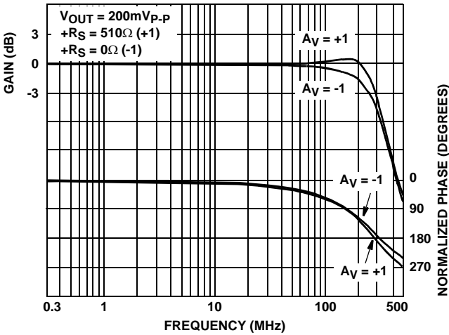
FIGURE 13. FREQUENCY RESPONSE
