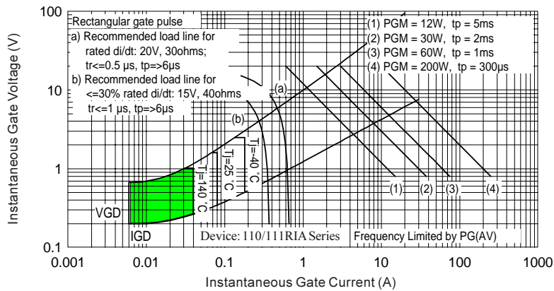
Fig. 9 - Gate Characteristics
