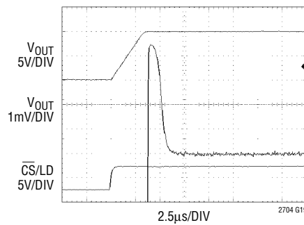
Settling 0V to 10V
