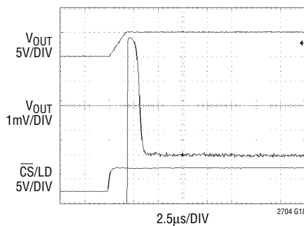
Settling 0V to 5V
