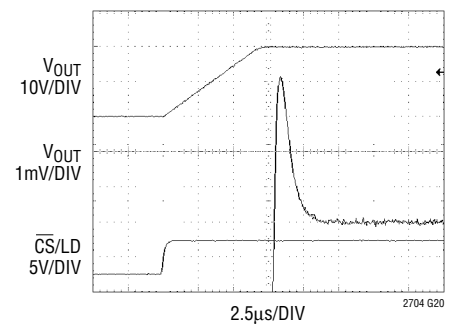
Settling ±10V
