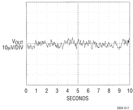
(LTC2604/LTC2604-1)
