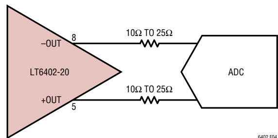
Figure 4. Adding Small Series R at LT6402 Output
