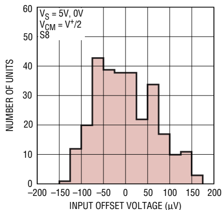
V_{\text{OS}} Distribution
