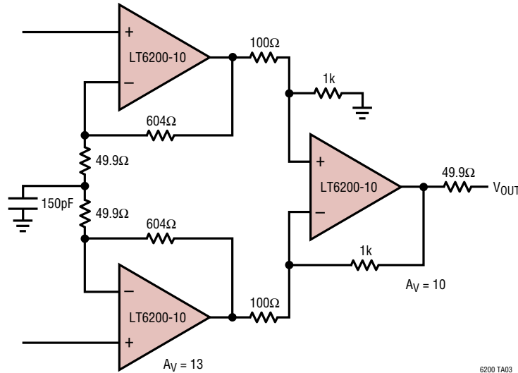
Rail-to-Rail High Speed Low Noise Instrumentation Amplifier
