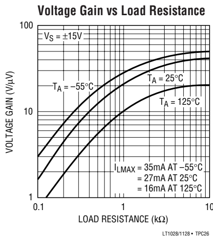
LT1028/1128 • TPC26
