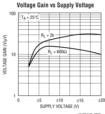
LT1028/1128 • TPC25
