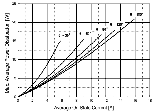
Fig 8. Power Dissipation
