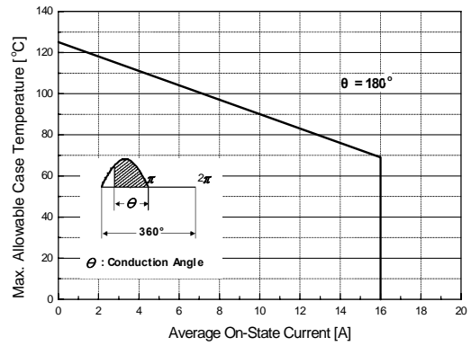
Fig 4. Thermal Response
