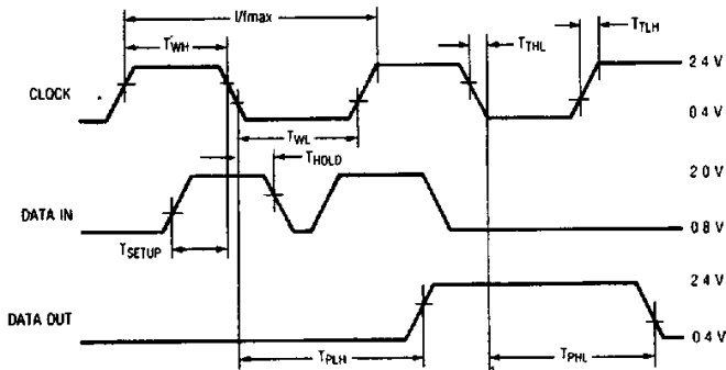
FIGURE 1. TIMING CHARACTERISTICS
