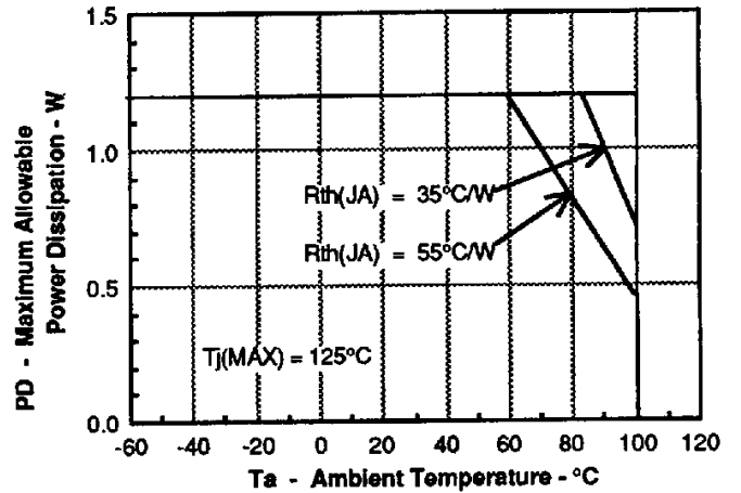
FIGURE 2. MAX. ALLOWABLE POWER DISSIPATION VS. TEMPERATURE
