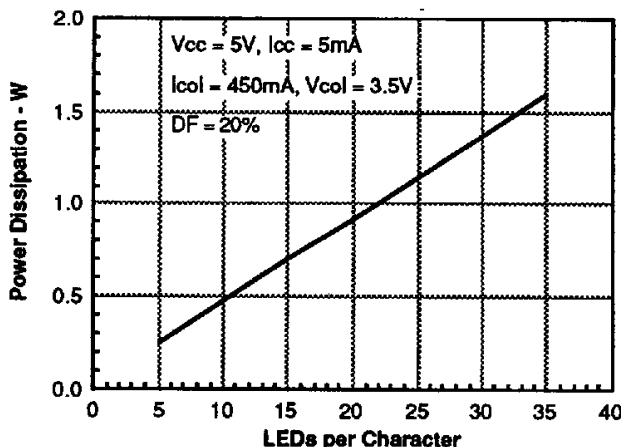
FIGURE 9. PACKAGE POWER DISSIPATION
