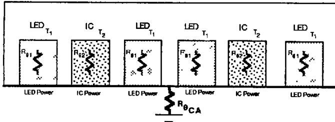
FIGURE 5. THERMAL MODEL
