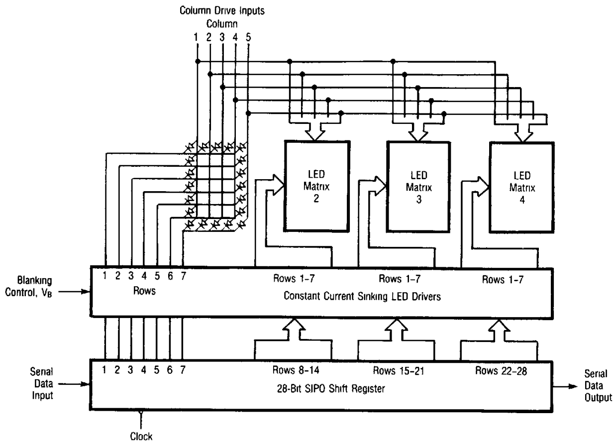
FIGURE 4. BLOCK DIAGRAM
