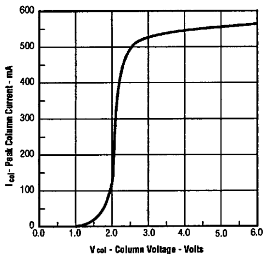
FIGURE 3. PEAK COLUMN CURRENT VS. COLUMN VOLTAGE
