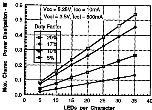
FIGURE 10. MAX. CHARACTER POWER DISSIPATION
