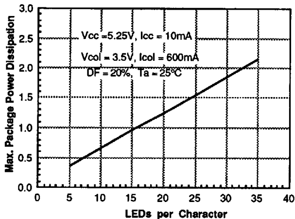
FIGURE 8. MAX. PACKAGE POWER DISSIPATION
