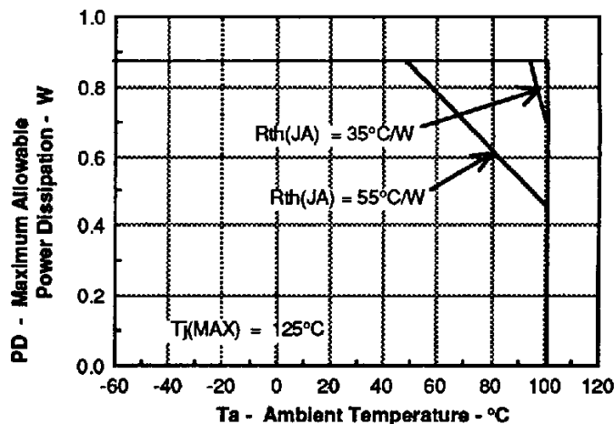
FIGURE 2. MAX. ALLOWABLE POWER DISSIPATION VS. TEMPERATURE
