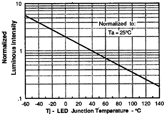
FIGURE 6. NORMALIZED LUMINOUS INTENSITY VS. JUNCTION TEMPERATURE
