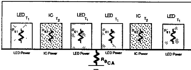
FIGURE 5. THERMAL MODEL
