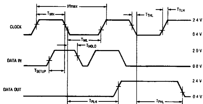
FIGURE 1. TIMING CHARACTERISTICS
