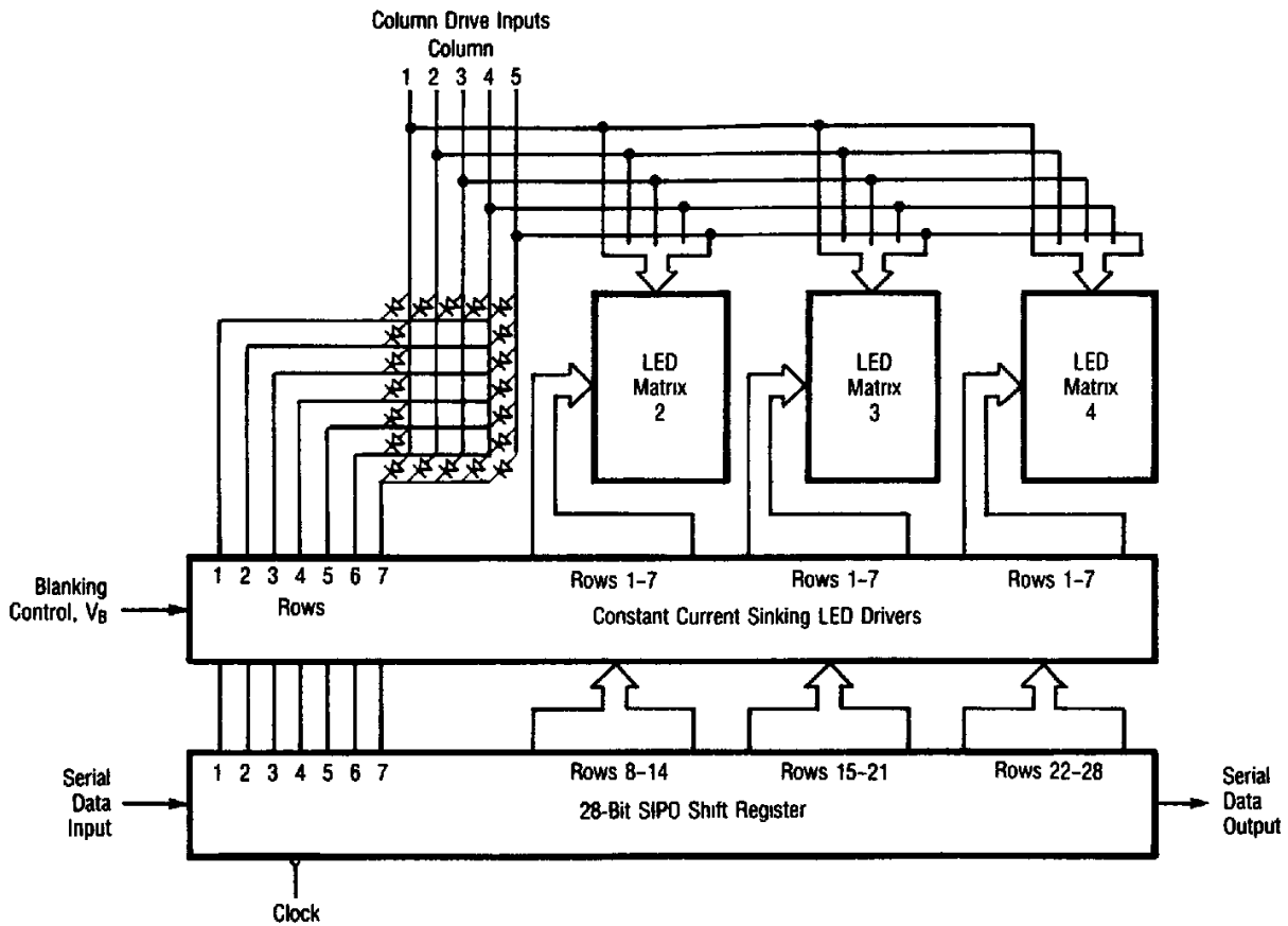
FIGURE 4. BLOCK DIAGRAM
