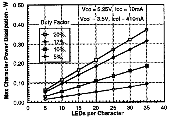
FIGURE 10. MAX. CHARACTER POWER DISSIPATION
