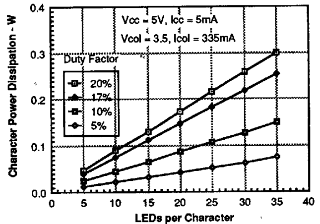
FIGURE 11. CHARACTER POWER DISSIPATION
