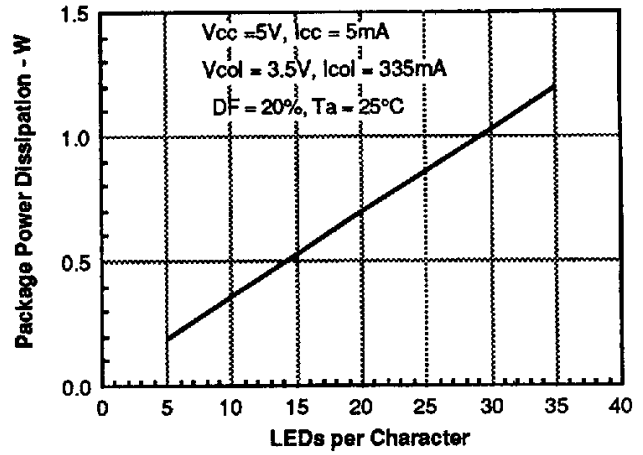
FIGURE 9. PACKAGE POWER DISSIPATION
