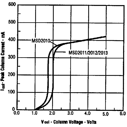
FIGURE 3. PEAK COLUMN CURRENT VS. COLUMN VOLTAGE
