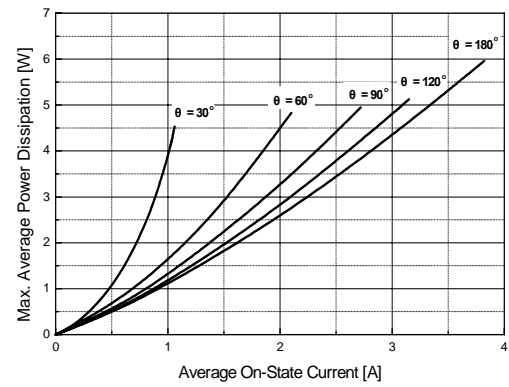
Fig 8. Power Dissipation
