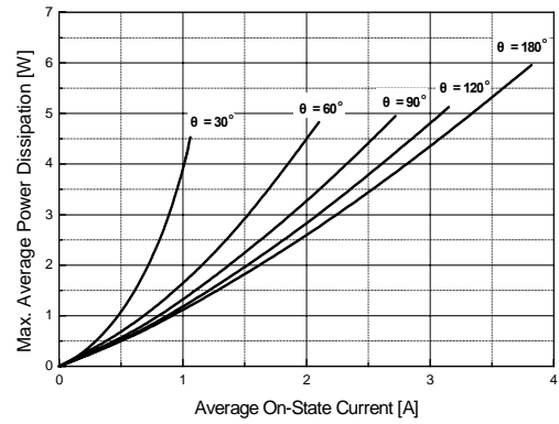
Fig 8. Power Dissipation
