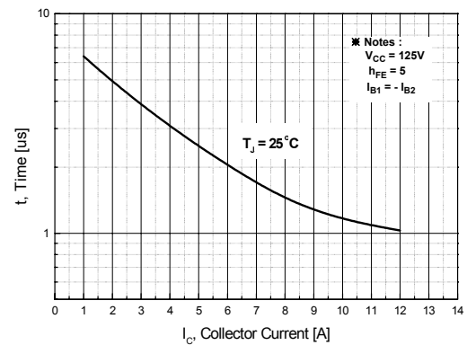
Fig 6. Resistive Load Storage Time
