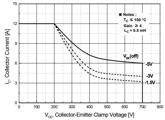
Fig 8. Reverse Biased Safe Operation Areas
