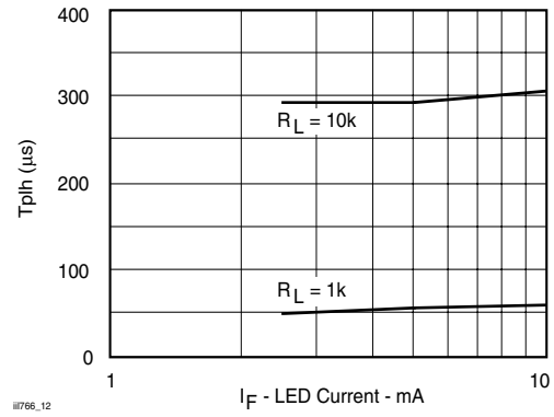
Figure 12. t_{\text{plh}} vs. Forward Current
