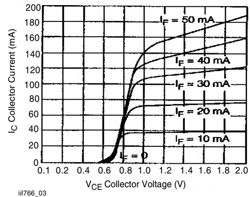
Figure 3. Transistor Output Current vs. Voltage
