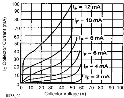
Figure 2. Transistor Current vs. Voltage
