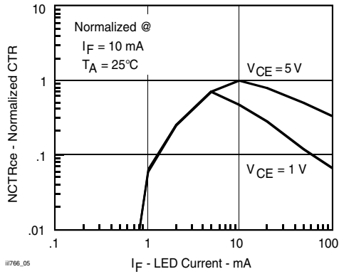
Figure 5. Normalized CTR vs. Forward Current
