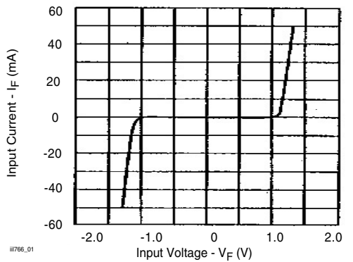
Figure 1. Input Characteristics
