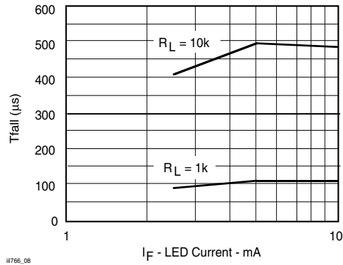
Figure 8. t_{fall} vs. Forward Current
