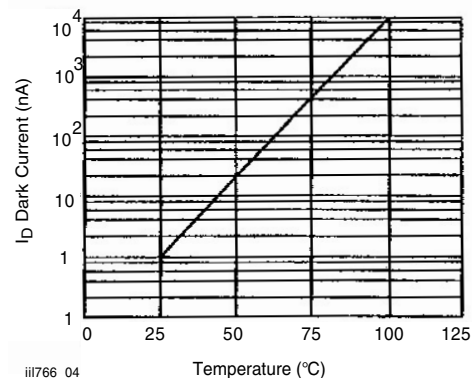
Figure 4. I_{CBO} at V_{CE} = 10 \text{ V} vs. Temperature
