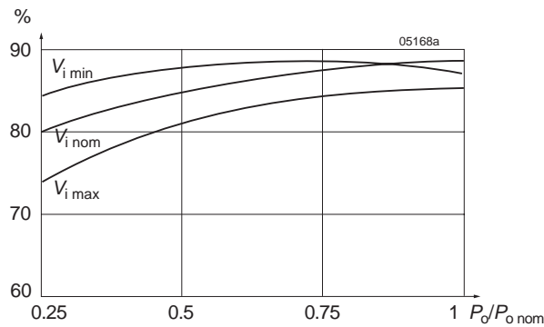
Fig. 11b Efficiency versus input voltage and load. Typical values (110IMY15-12-12-8)
