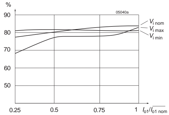
Fig. 12 Efficiency versus input voltage and load. Typical values (48IMS15-12-12-9)
