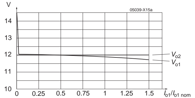
Fig. 13 Flexible load distribution on double-outputs models with option R (110IMY15-12-12-8R): Load variation from 0 to 150% of I_{o1 nom} on output 1; output 2 loaded with 50% of I_{o2 nom} .
