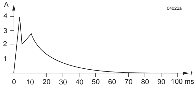
Fig. 4 Typical inrush current at V_{i\text{nom}} , P_{o\text{nom}} versus time (40IMX15). Source impedance according to ETS 300132-2 at V_{i\text{nom}} .
