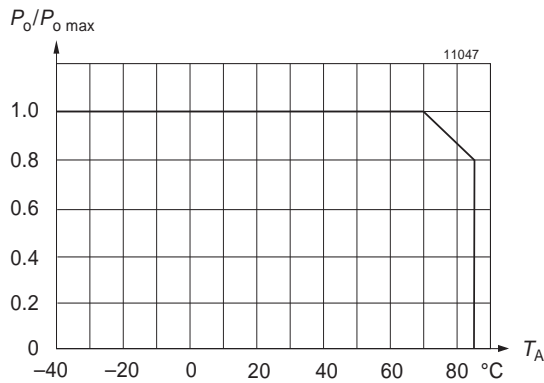
Fig. 23 Maximum allowed output power versus ambient temperature.
