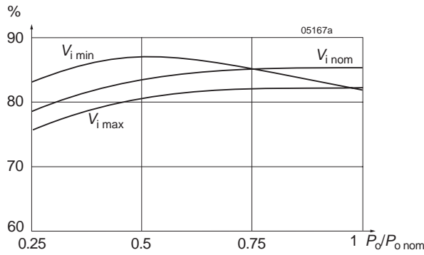
Fig. 11a Efficiency versus input voltage and load. Typical values (40IMX15-12-12-8).
