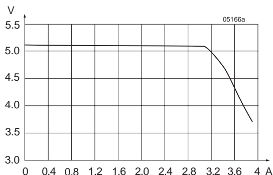
Fig. 8 V_o versus I_o (typ) of converters with V_o = 5.1 \text{ V} (110IMY15-05-8R)
