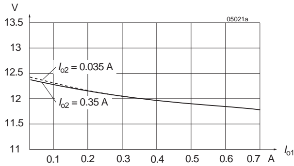
Fig. 10 Cross load regulation V_{o1} versus I_{o1} (typ.) for various I_{o2} ( 2 \times 12 V).
