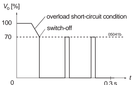
Fig. 7 Overload switch-off (hiccup mode); typical values
