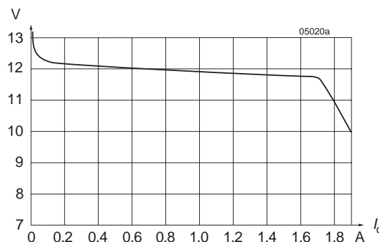
Fig. 9 V_o versus I_o (typ.) of double-output models (2 x 12 V), with both outputs in parallel (110IMY15-12-12-8)
