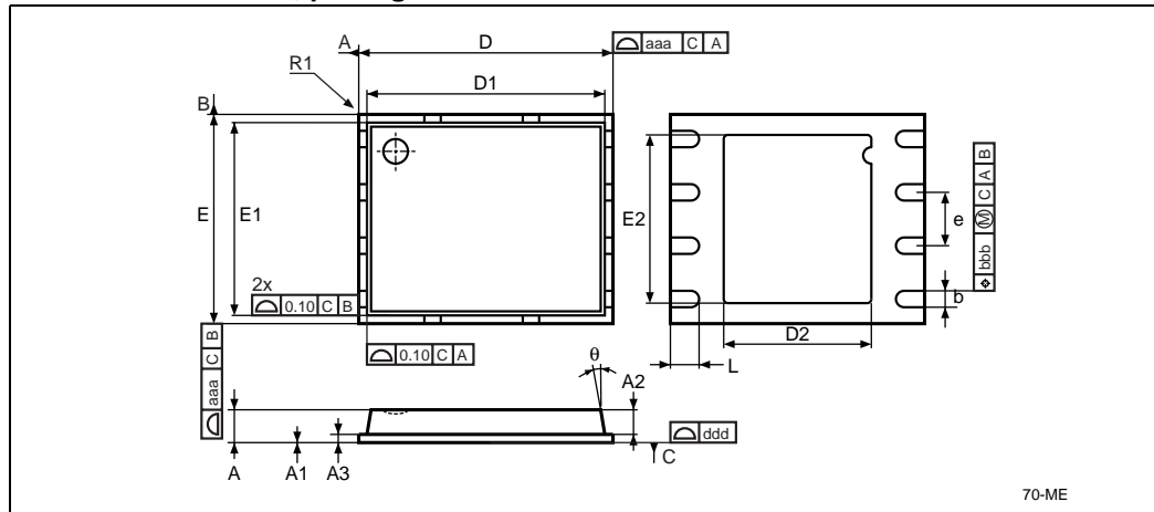
Figure 34. VFQFPN8 (MLP8) 8-lead very thin fine pitch quad flat package no lead, 6 × 5 mm, package outline
