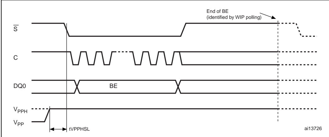
Figure 33. V_{PPH} timing
